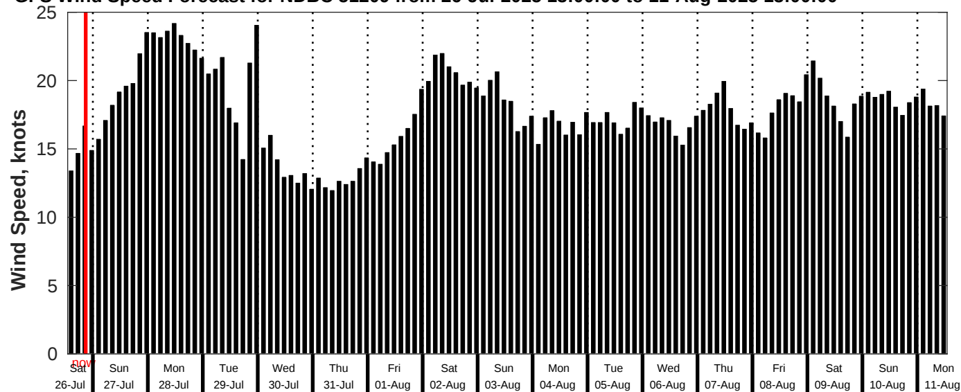
GFS Wind Speed Forecast for NDBC 51209 from 26-Jul-2025 13:00:00 to 11-Aug-2025 13:00:00
