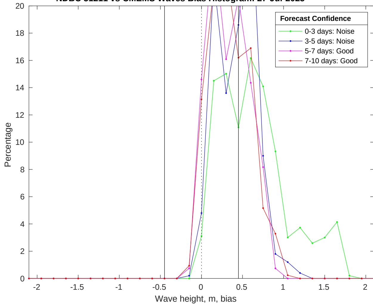
NDBC 51211 vs CMEMS Waves Bias Histogram: 27-Jul-2025
