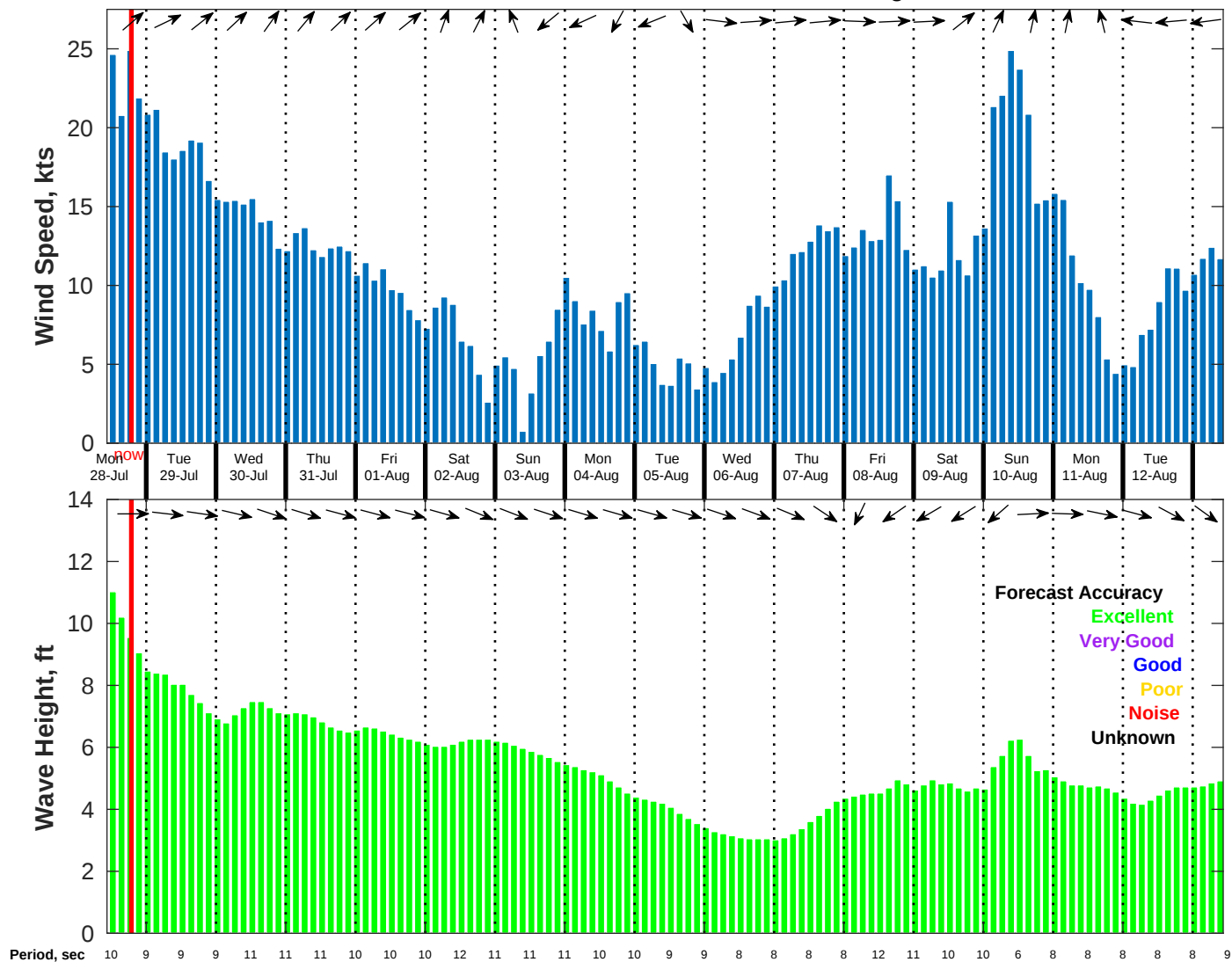
Wind & Wave Forecast for NDBC 52211 from 27-Jul-2025 11:00:00 to 12-Aug-2025 11:00:00
