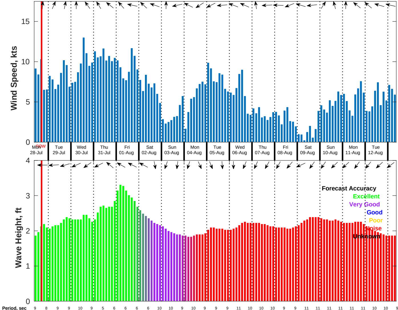
Wind & Wave Forecast for NDBC 52212 from 27-Jul-2025 09:00:00 to 12-Aug-2025 09:00:00
