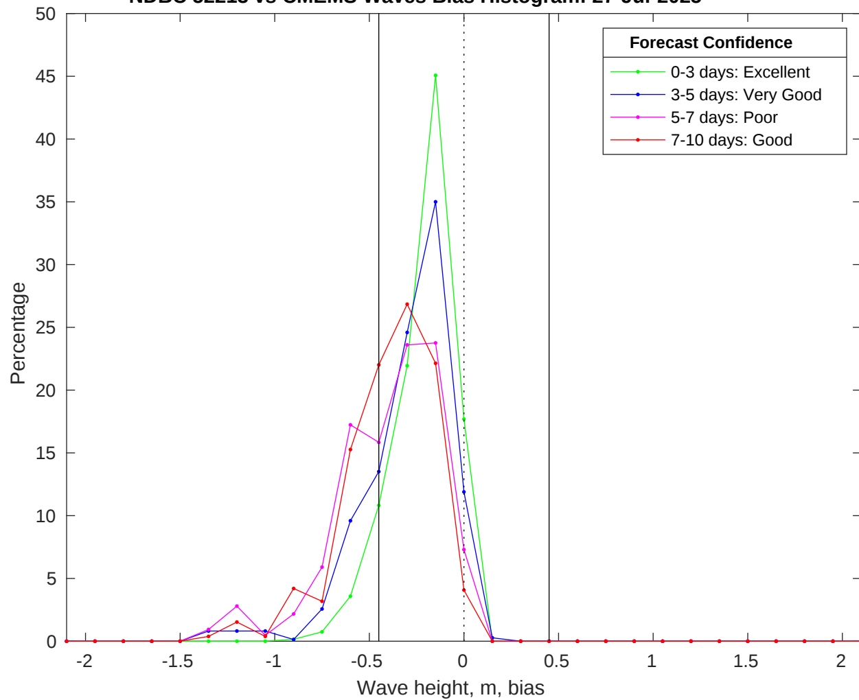
NDBC 52213 vs CMEMS Waves Bias Histogram: 27-Jul-2025
