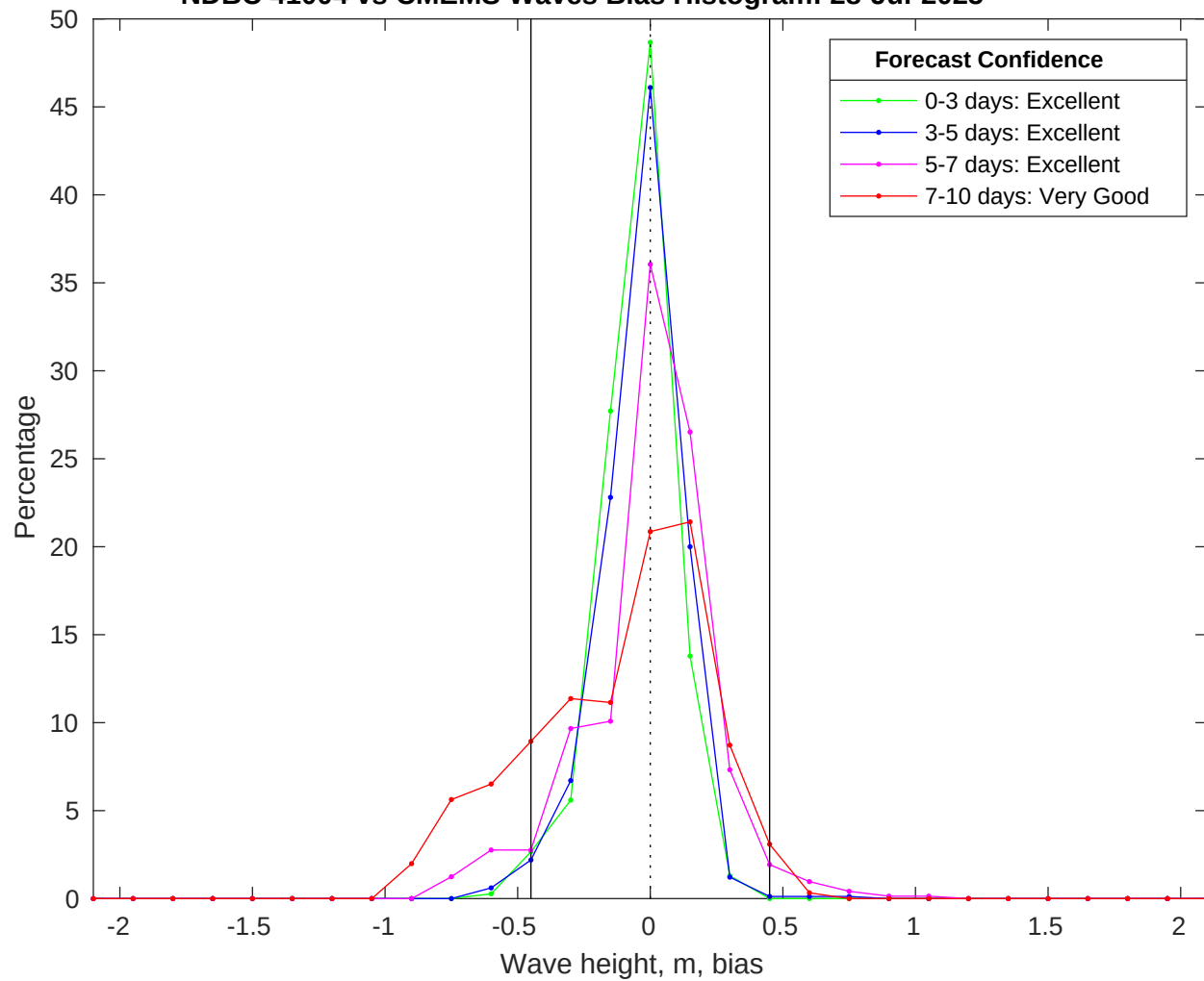
NDBC 41004 vs CMEMS Waves Bias Histogram: 28-Jul-2025
