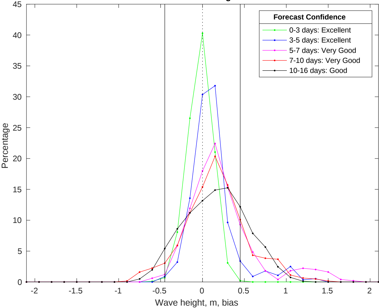
NDBC 41004 vs GFS Waves Bias Histogram: 28-Jul-2025
