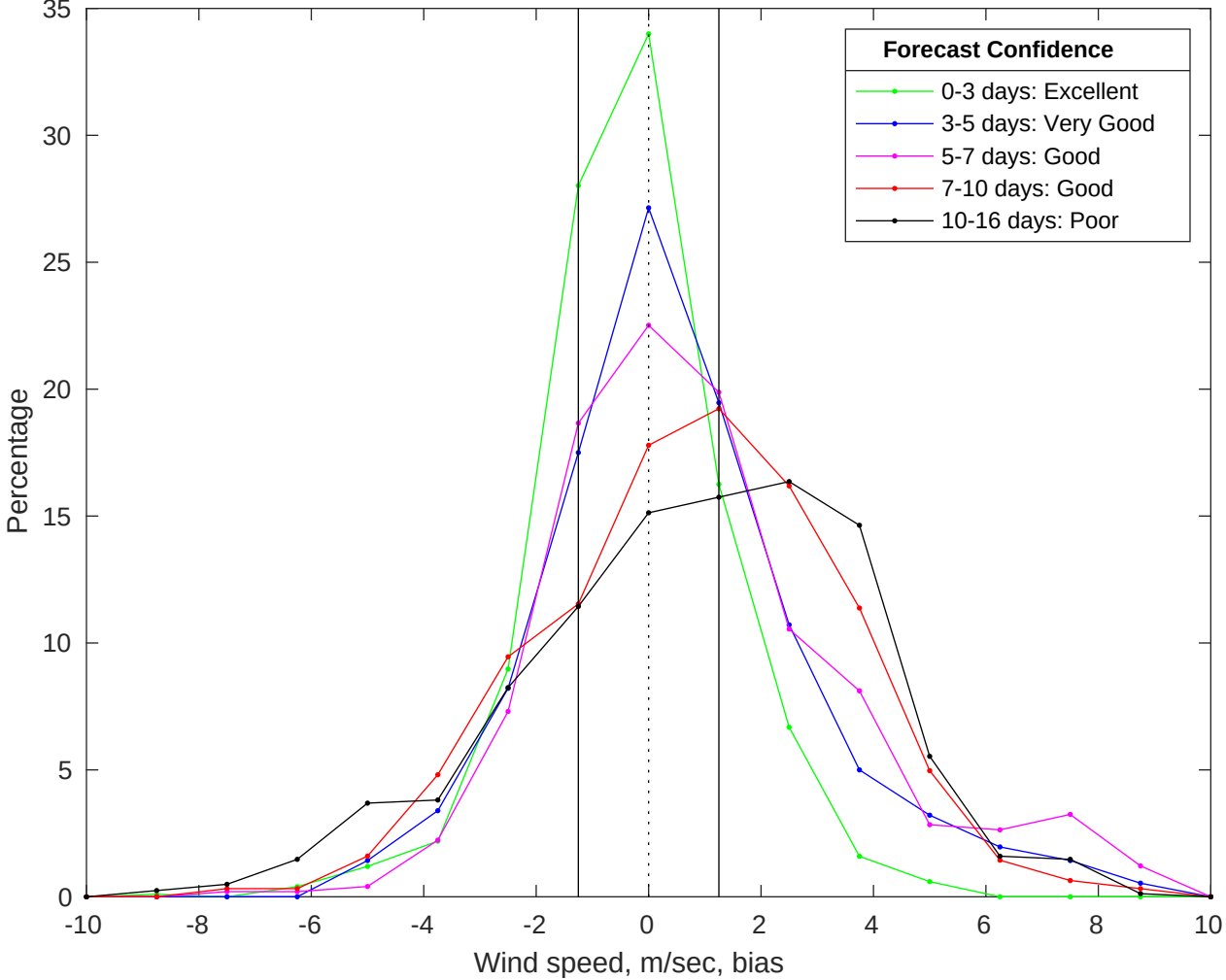
NDBC 41004 vs GFS Winds Bias Histogram: 28-Jul-2025
