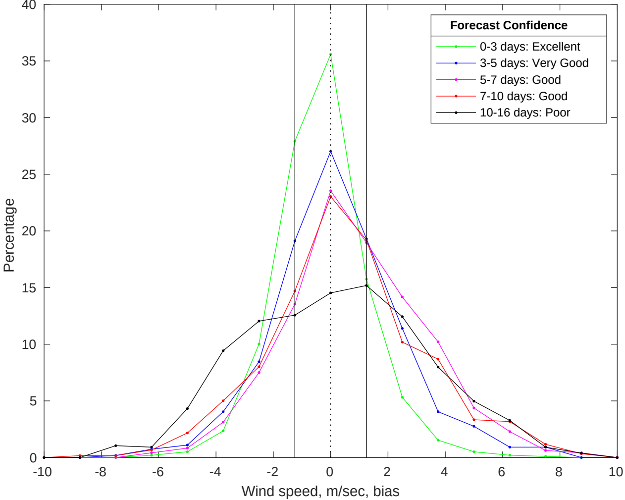
NDBC 41013 vs GFS Winds Bias Histogram: 28-Jul-2025
