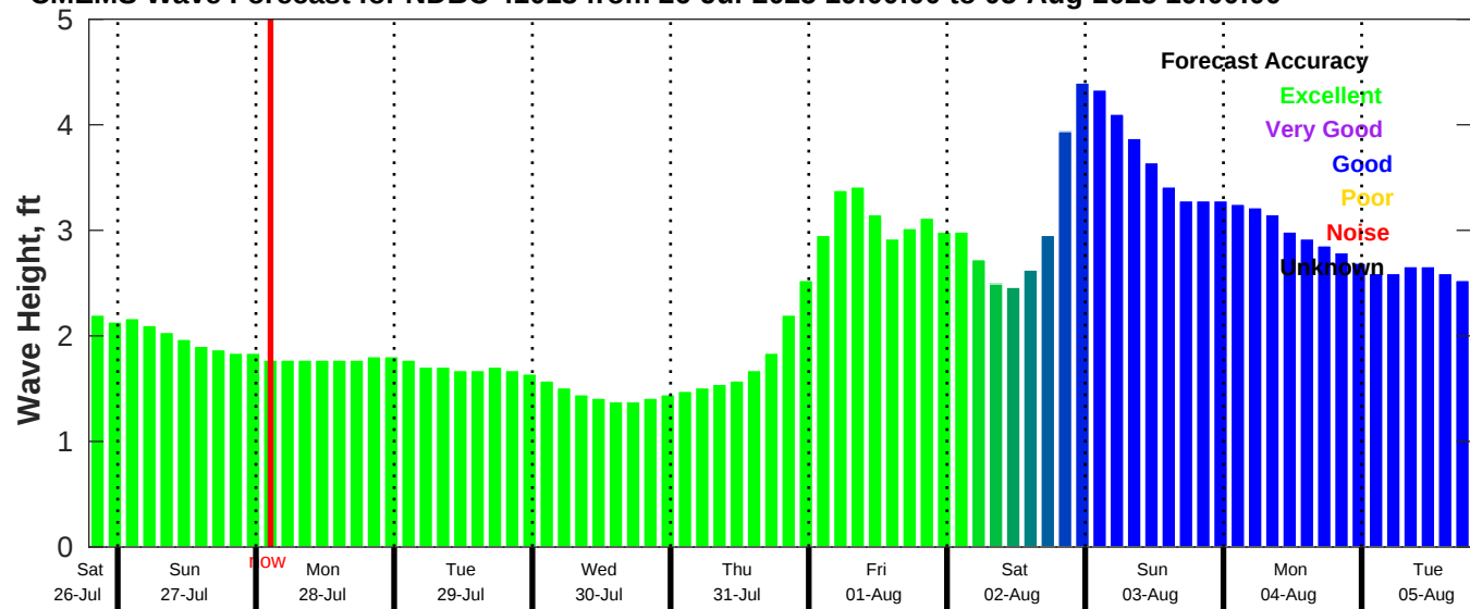
CMEMS Wave Forecast for NDBC 41013 from 26-Jul-2025 19:00:00 to 05-Aug-2025 19:00:00
