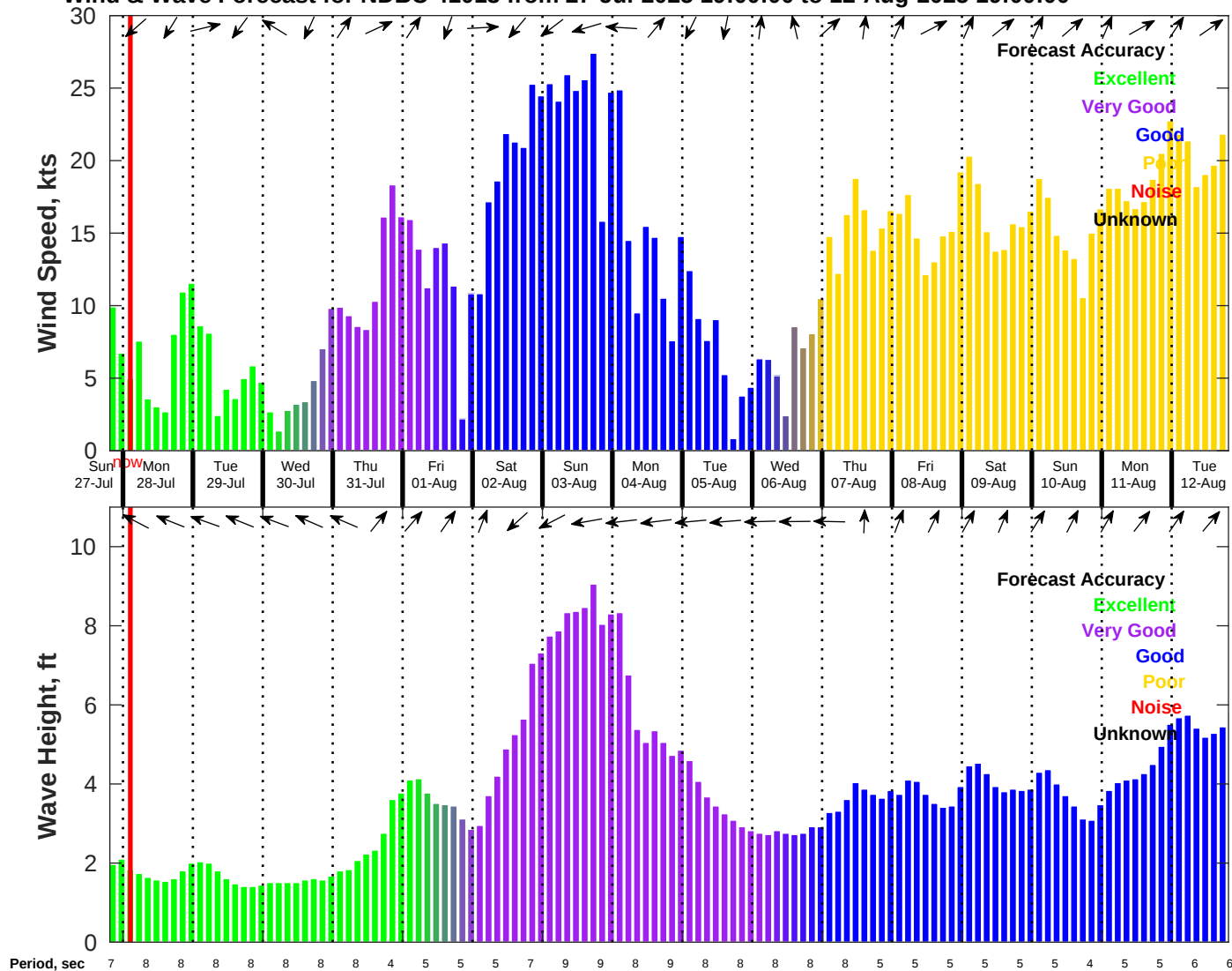
Wind & Wave Forecast for NDBC 41013 from 27-Jul-2025 19:00:00 to 12-Aug-2025 19:00:00
