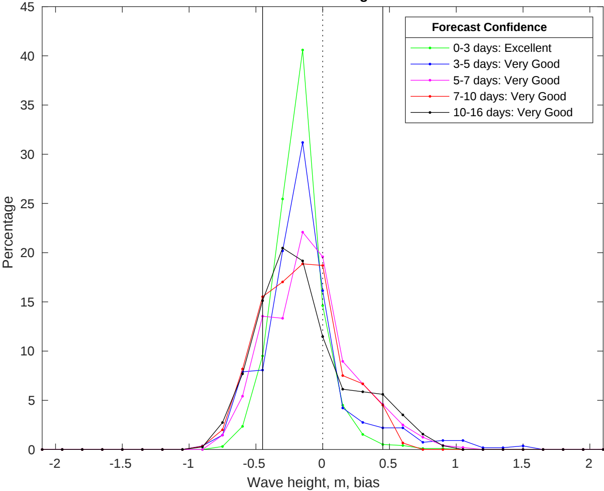
NDBC 41040 vs GFS Waves Bias Histogram: 28-Jul-2025
