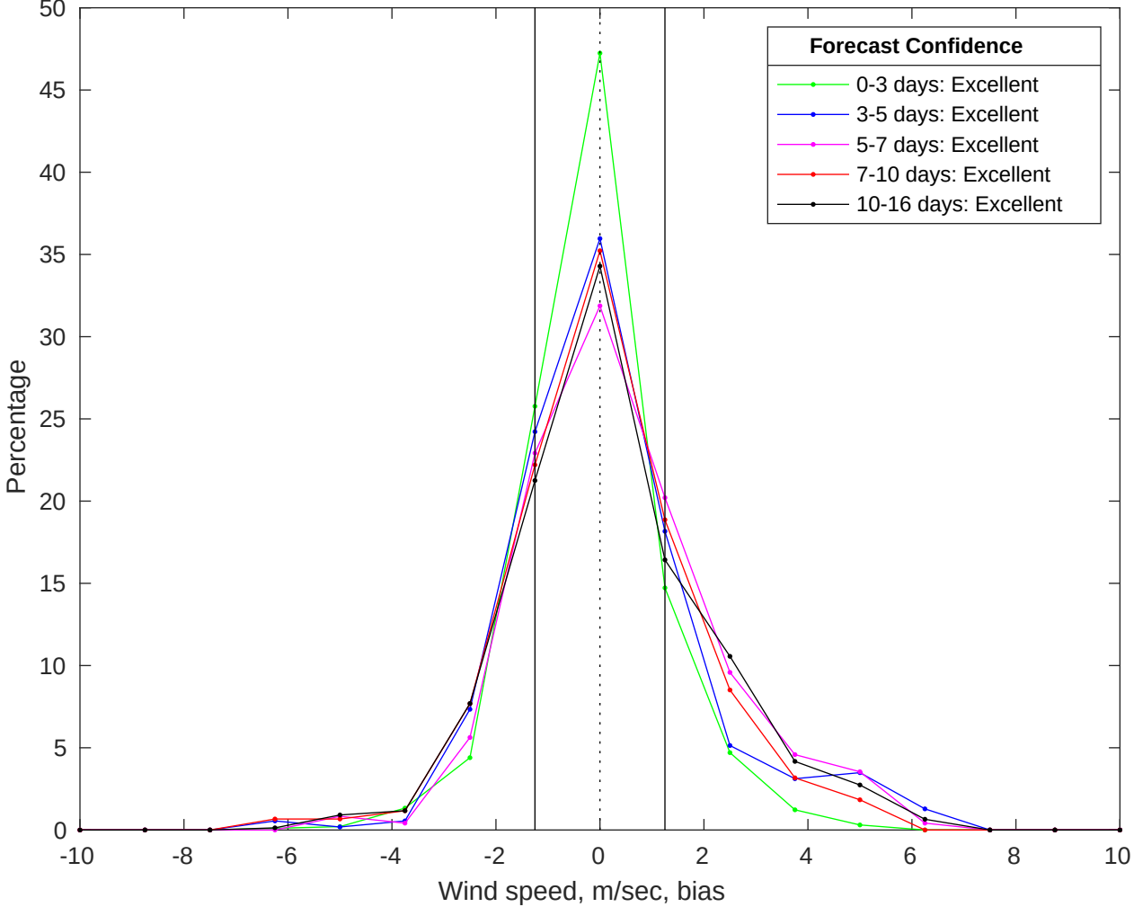
NDBC 41040 vs GFS Winds Bias Histogram: 28-Jul-2025
