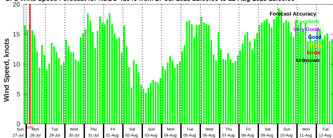
GFS Wind Speed Forecast for NDBC 41040 from 27-Jul-2025 21:00:00 to 12-Aug-2025 21:00:00
