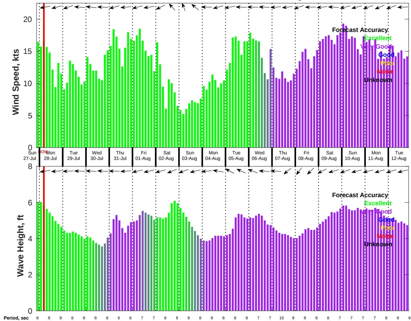
Wind & Wave Forecast for NDBC 41040 from 27-Jul-2025 21:00:00 to 12-Aug-2025 21:00:00
