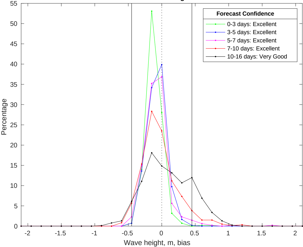
NDBC 42019 vs GFS Waves Bias Histogram: 28-Jul-2025
