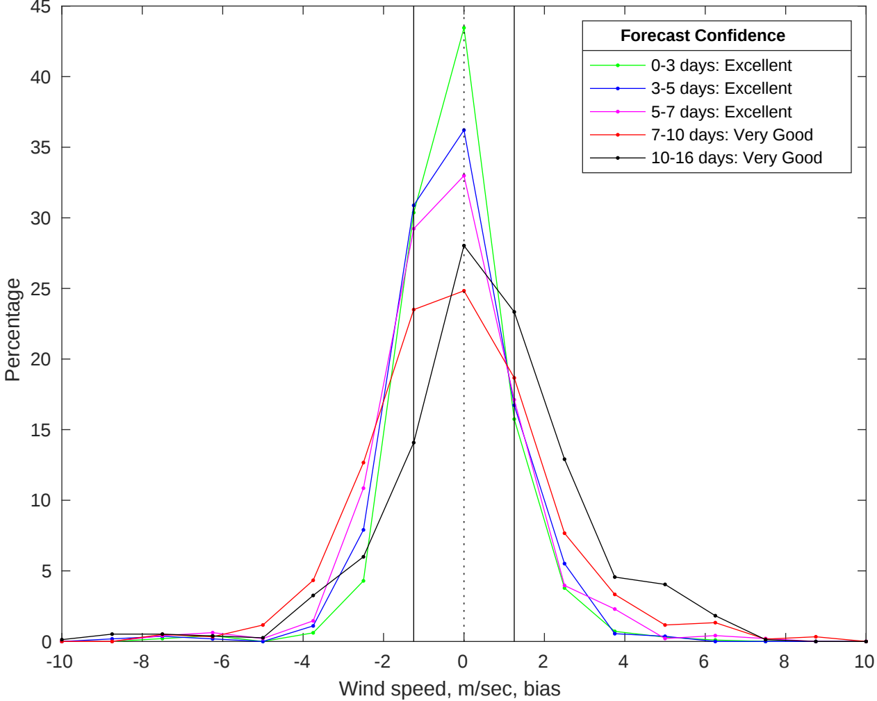
NDBC 42019 vs GFS Winds Bias Histogram: 28-Jul-2025
