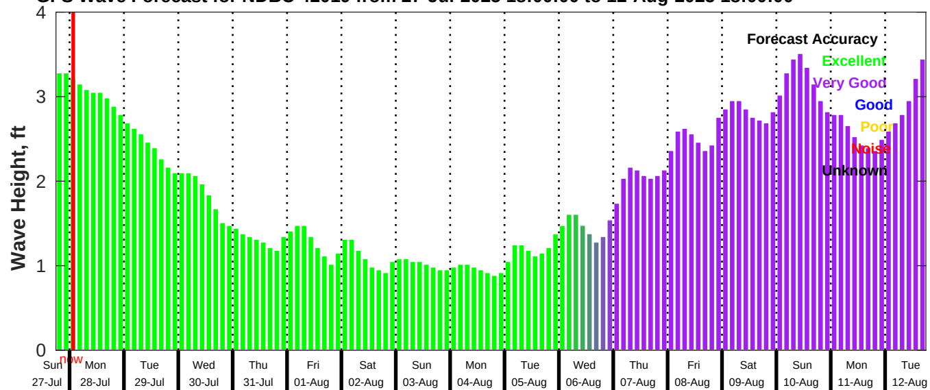
GFS Wave Forecast for NDBC 42019 from 27-Jul-2025 18:00:00 to 12-Aug-2025 18:00:00
