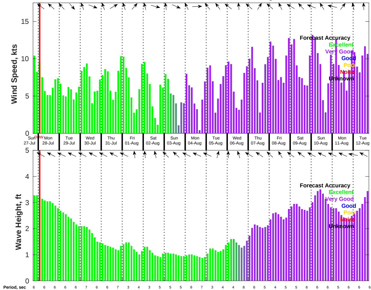
Wind & Wave Forecast for NDBC 42019 from 27-Jul-2025 18:00:00 to 12-Aug-2025 18:00:00
