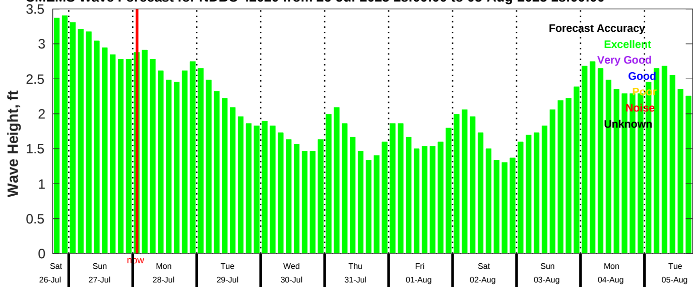
CMEMS Wave Forecast for NDBC 42020 from 26-Jul-2025 18:00:00 to 05-Aug-2025 18:00:00
