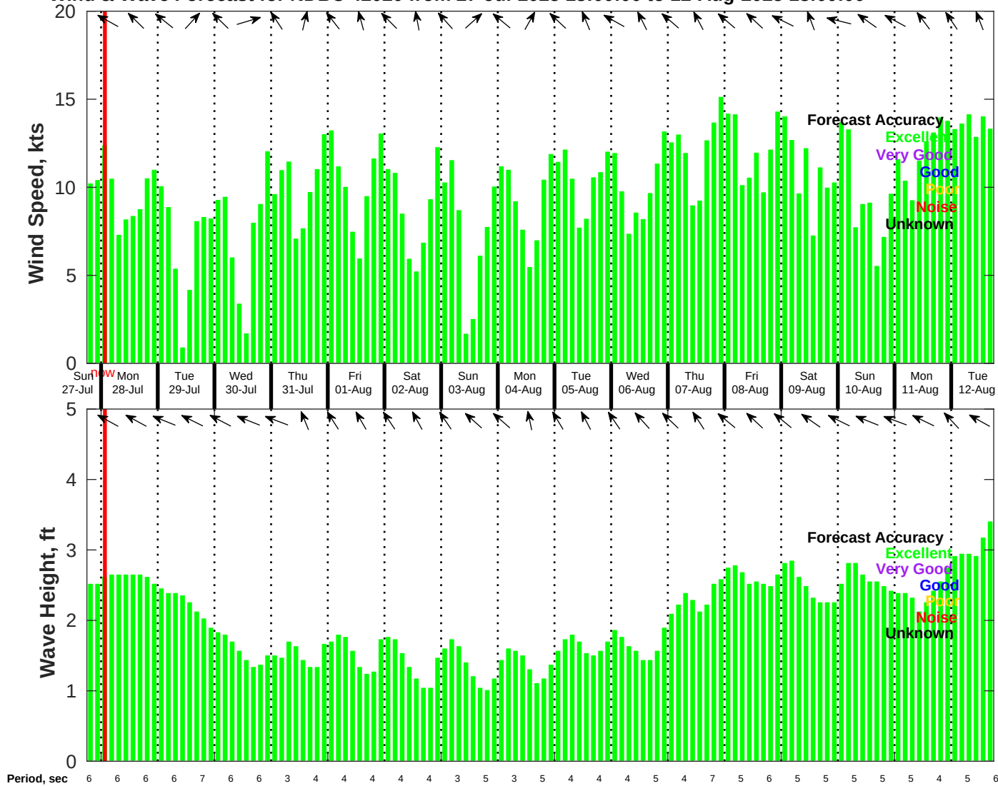
Wind & Wave Forecast for NDBC 42020 from 27-Jul-2025 18:00:00 to 12-Aug-2025 18:00:00
