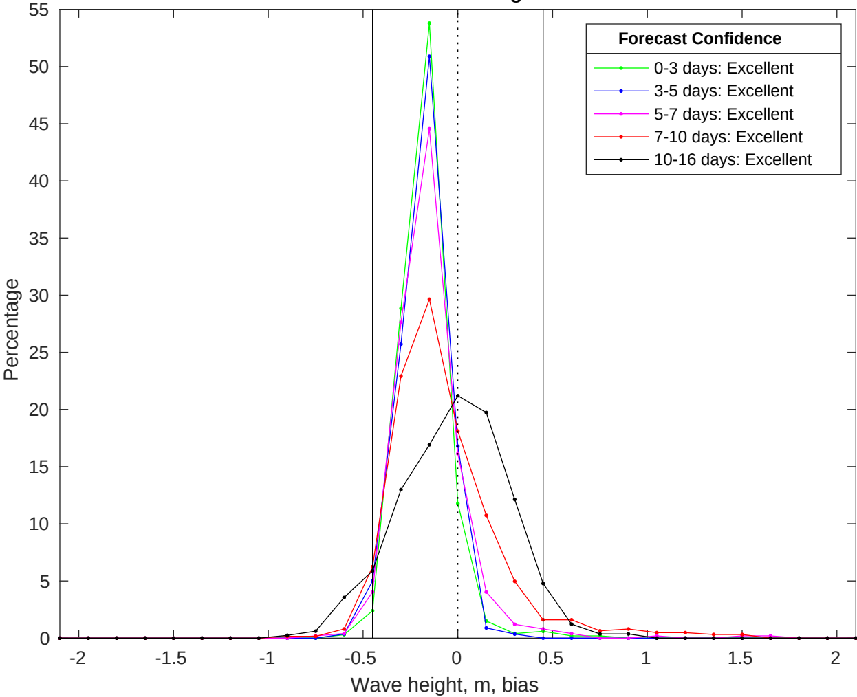
NDBC 42035 vs GFS Waves Bias Histogram: 28-Jul-2025
