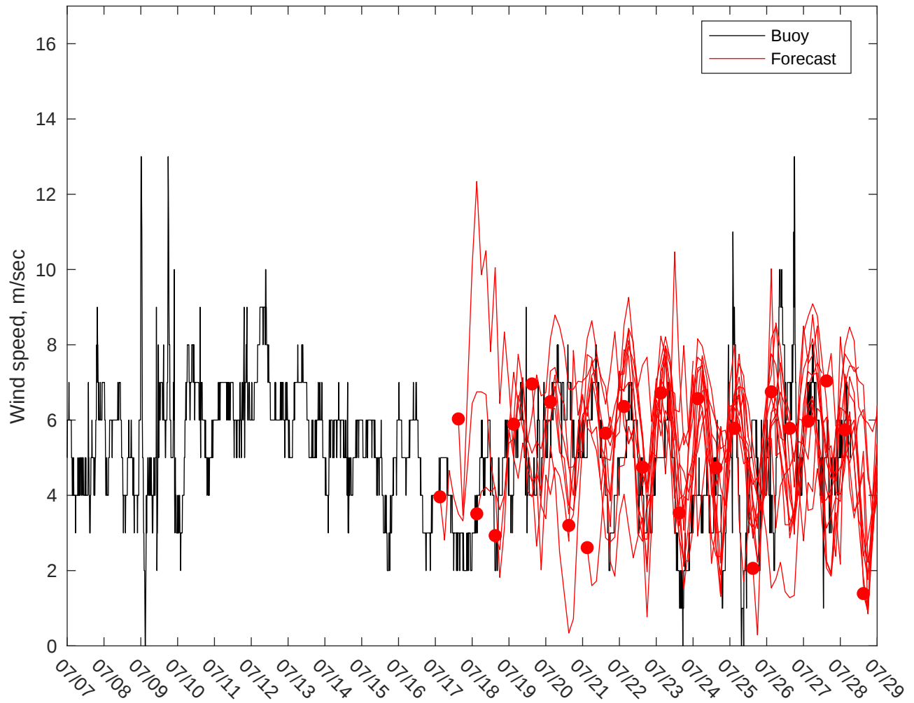
NDBC 42035 vs GFS Winds: 10 to 16 day forecast
