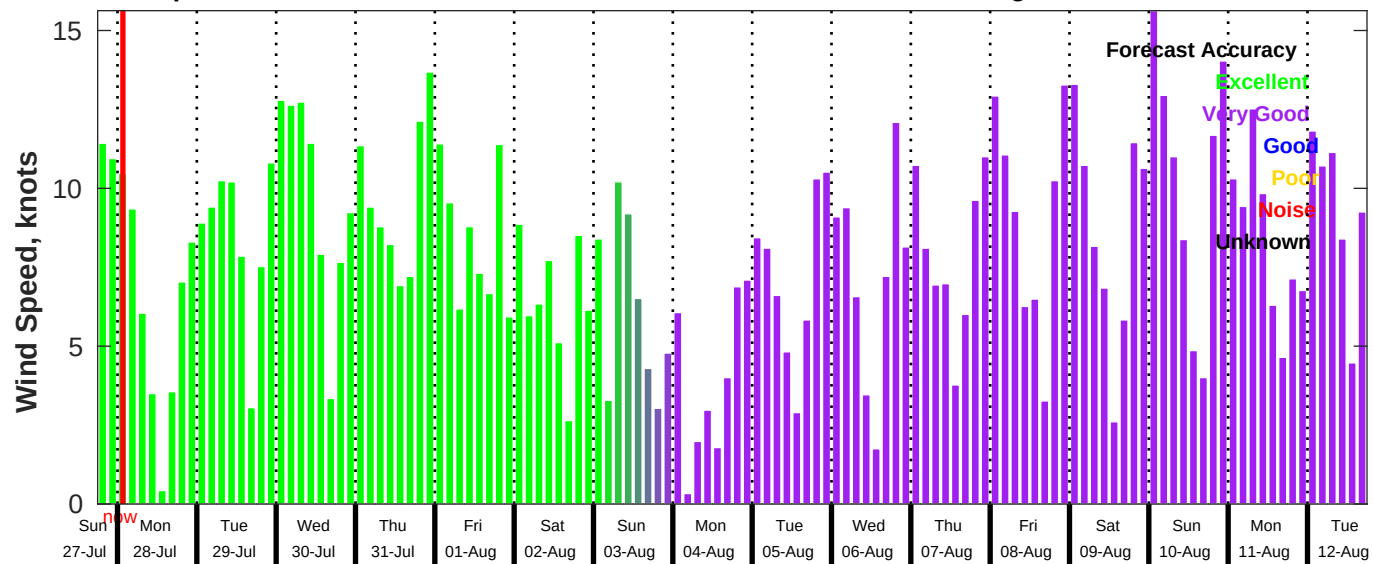
GFS Wind Speed Forecast for NDBC 42035 from 27-Jul-2025 18:00:00 to 12-Aug-2025 18:00:00
