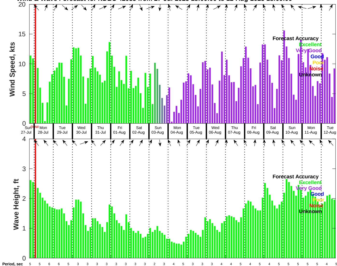
Wind & Wave Forecast for NDBC 42035 from 27-Jul-2025 18:00:00 to 12-Aug-2025 18:00:00
