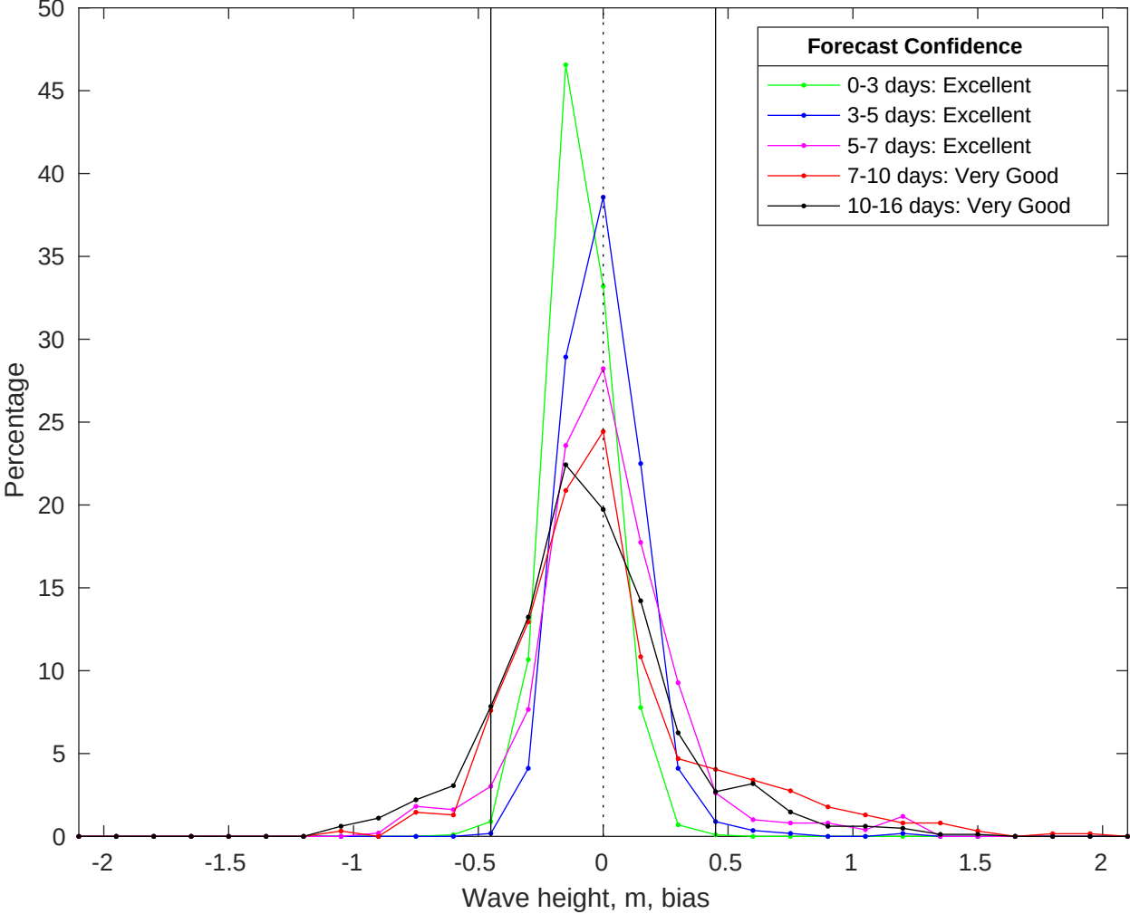
NDBC 42036 vs GFS Waves Bias Histogram: 28-Jul-2025
