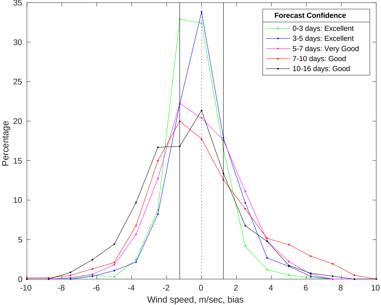
NDBC 42036 vs GFS Winds Bias Histogram: 28-Jul-2025
