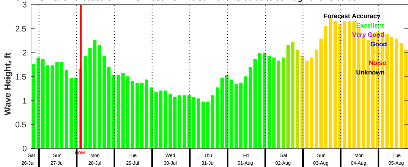
CMEMS Wave Forecast for NDBC 42036 from 26-Jul-2025 19:00:00 to 05-Aug-2025 19:00:00
