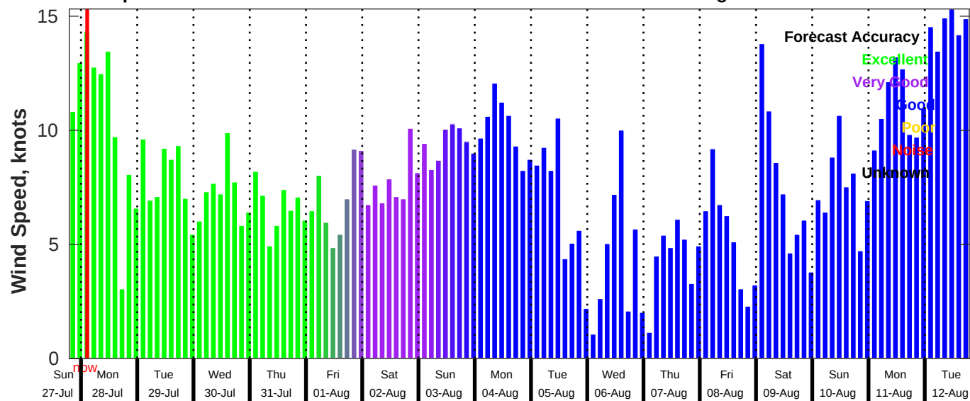
GFS Wind Speed Forecast for NDBC 42036 from 27-Jul-2025 19:00:00 to 12-Aug-2025 19:00:00
