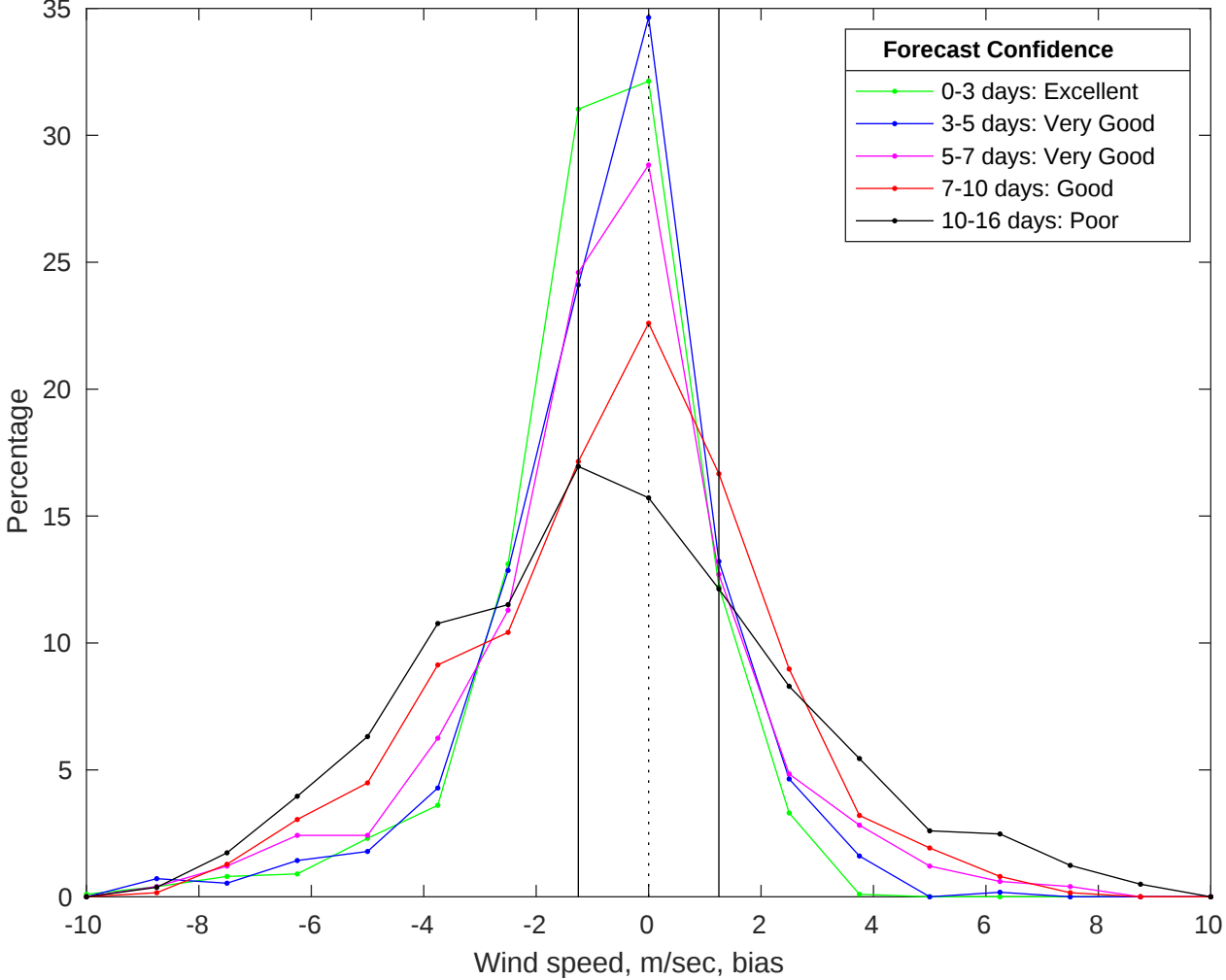
NDBC 42040 vs GFS Winds Bias Histogram: 28-Jul-2025
