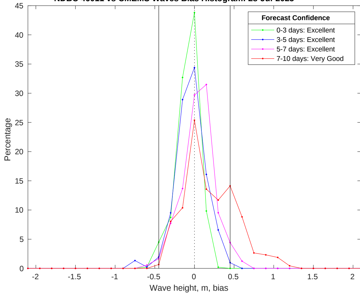
NDBC 46011 vs CMEMS Waves Bias Histogram: 28-Jul-2025
