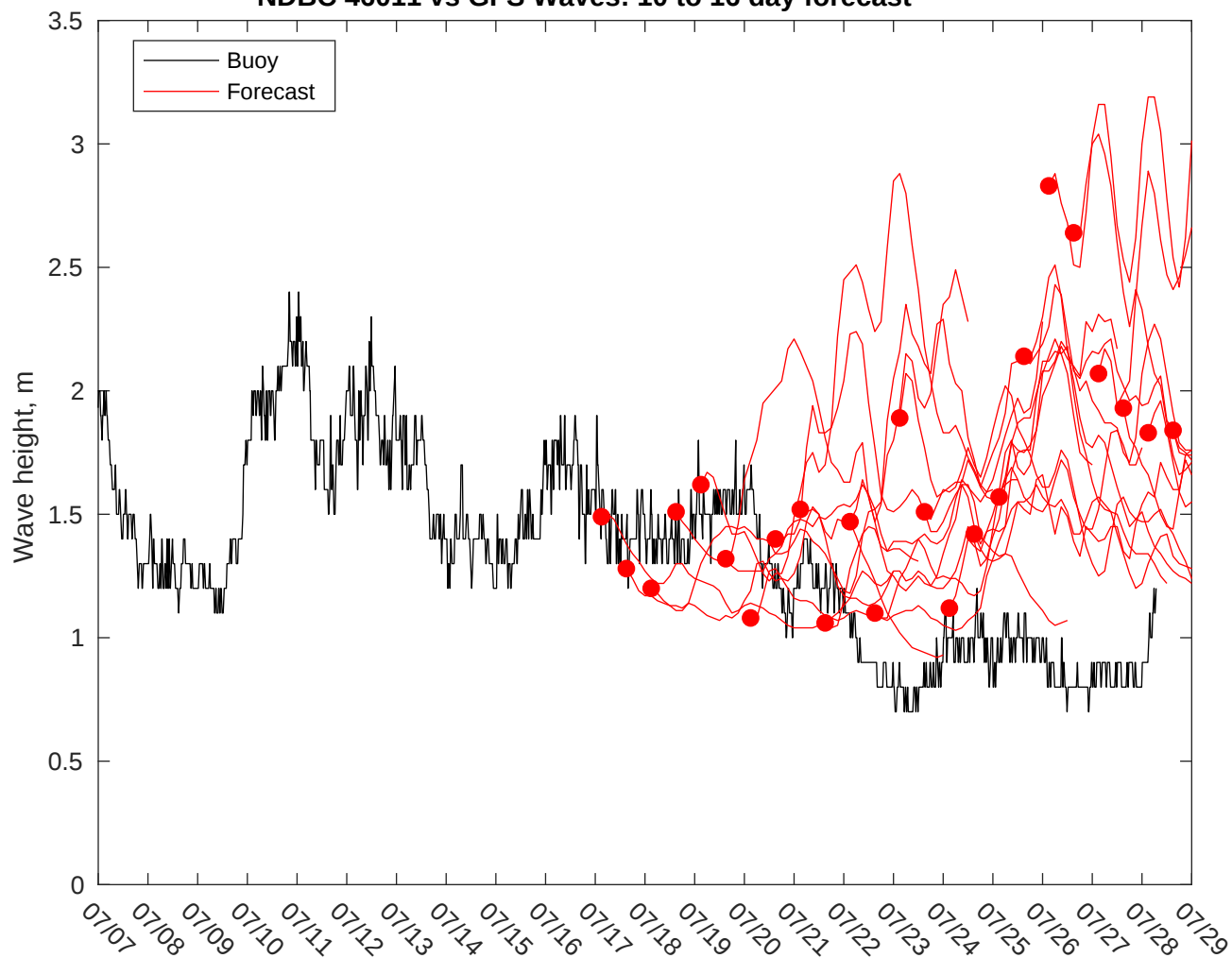
NDBC 46011 vs GFS Waves: 10 to 16 day forecast
