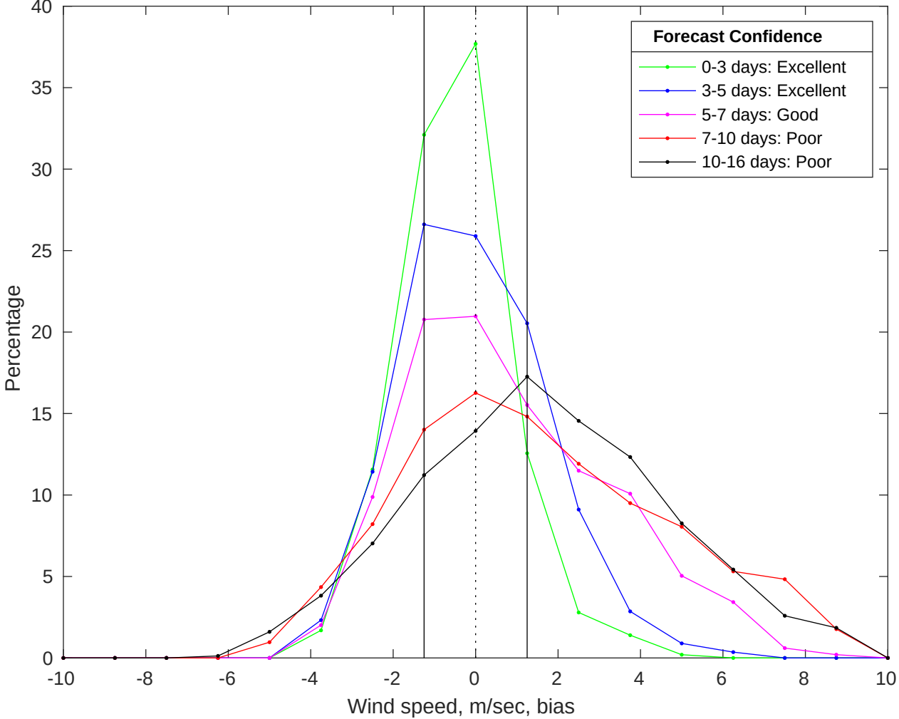
NDBC 46011 vs GFS Winds Bias Histogram: 28-Jul-2025
