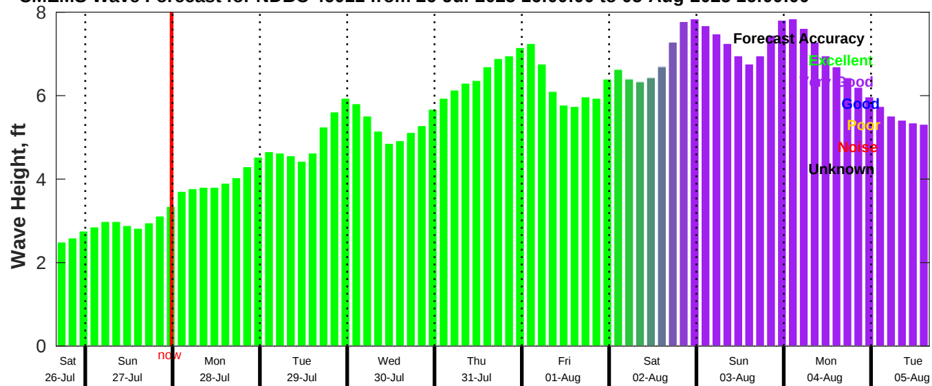
CMEMS Wave Forecast for NDBC 46011 from 26-Jul-2025 16:00:00 to 05-Aug-2025 16:00:00
