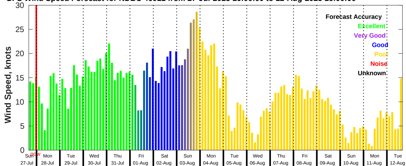
GFS Wind Speed Forecast for NDBC 46011 from 27-Jul-2025 16:00:00 to 12-Aug-2025 16:00:00
