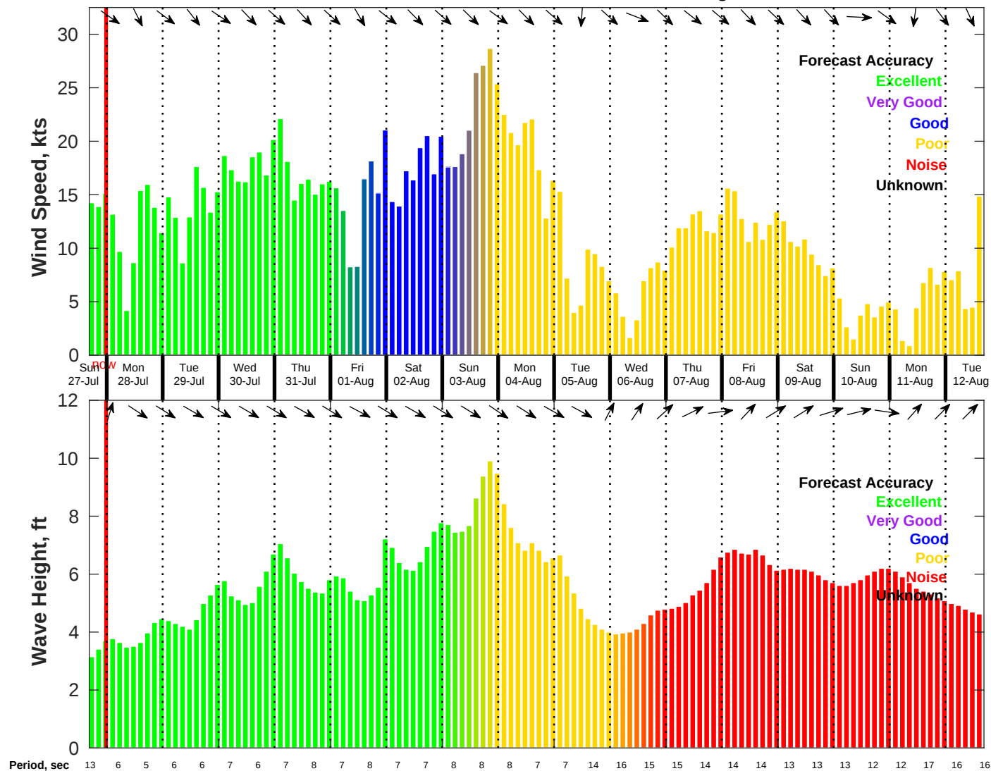
Wind & Wave Forecast for NDBC 46011 from 27-Jul-2025 16:00:00 to 12-Aug-2025 16:00:00
