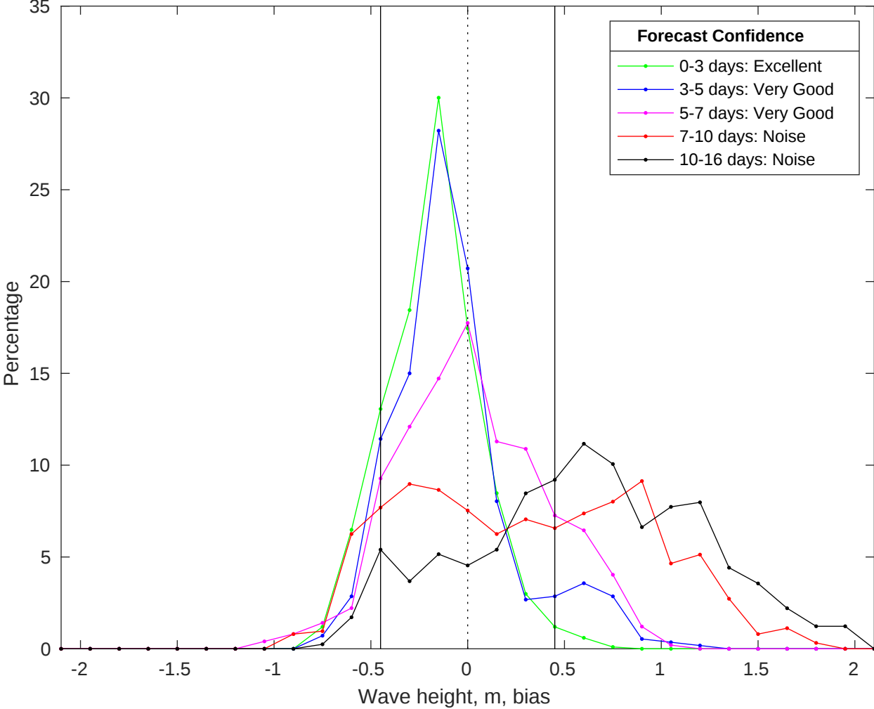
NDBC 46028 vs GFS Waves Bias Histogram: 28-Jul-2025
