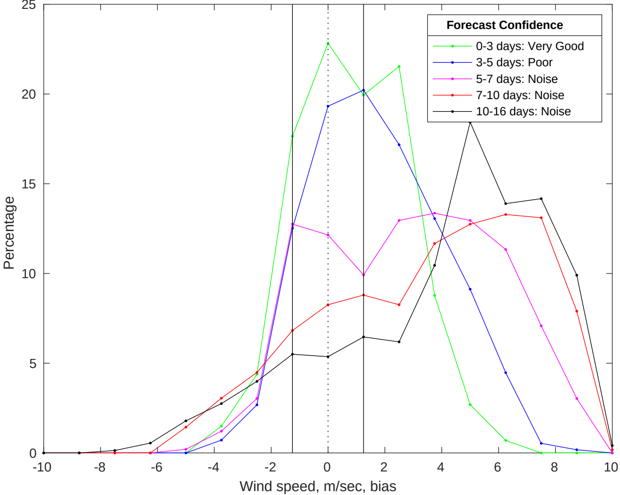
NDBC 46028 vs GFS Winds Bias Histogram: 28-Jul-2025
