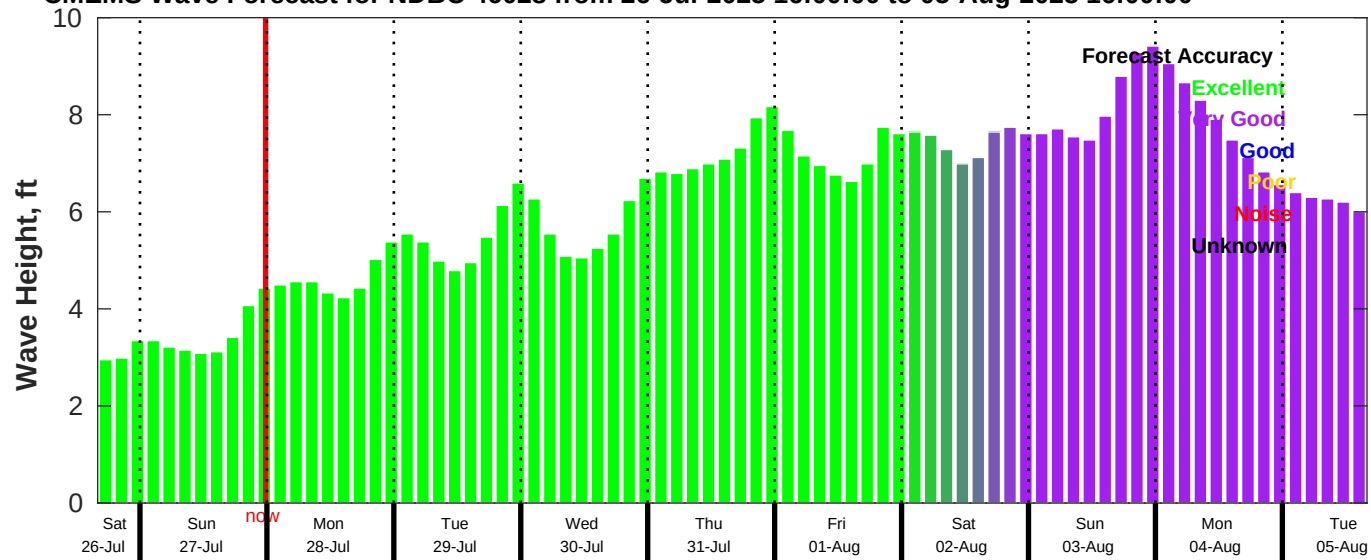
CMEMS Wave Forecast for NDBC 46028 from 26-Jul-2025 16:00:00 to 05-Aug-2025 16:00:00
