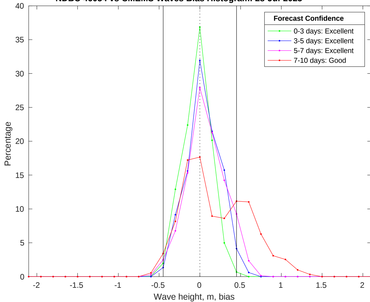
NDBC 46054 vs CMEMS Waves Bias Histogram: 28-Jul-2025
