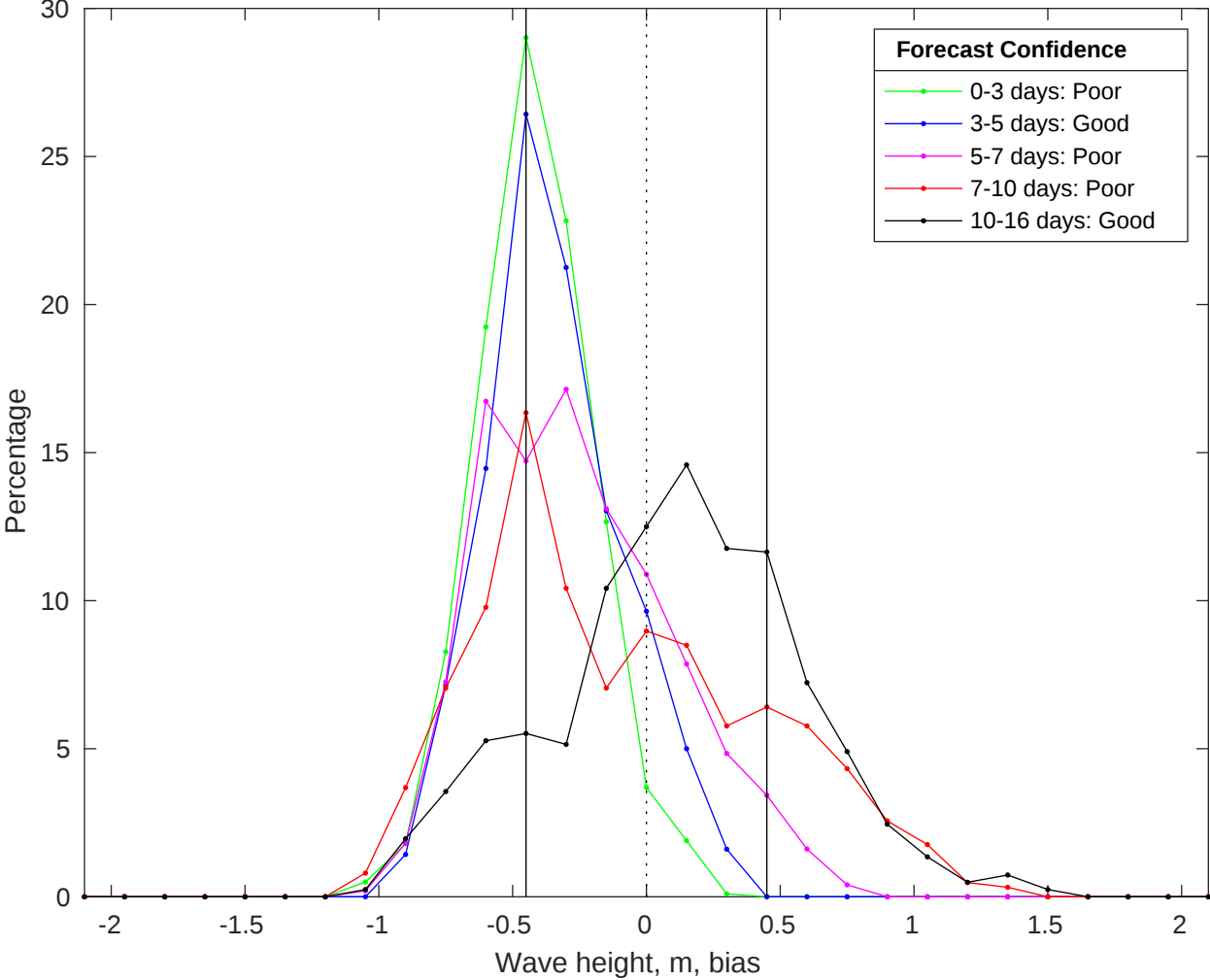
NDBC 46054 vs GFS Waves Bias Histogram: 28-Jul-2025
