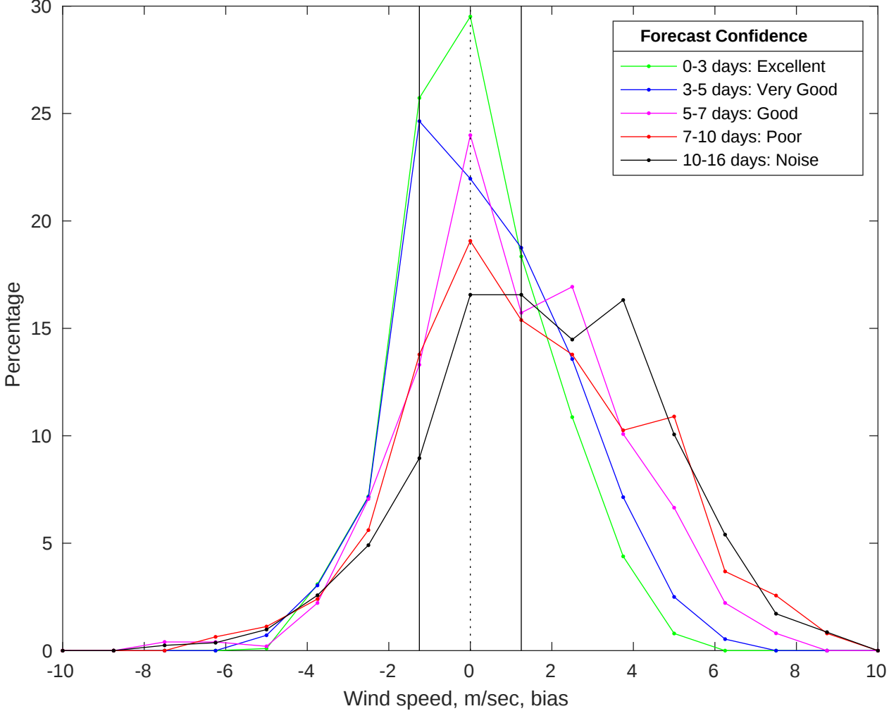
NDBC 46054 vs GFS Winds Bias Histogram: 28-Jul-2025
