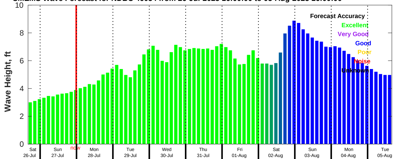
CMEMS Wave Forecast for NDBC 46054 from 26-Jul-2025 16:00:00 to 05-Aug-2025 16:00:00
