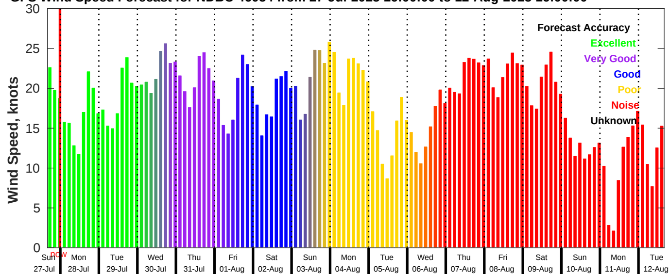
GFS Wind Speed Forecast for NDBC 46054 from 27-Jul-2025 16:00:00 to 12-Aug-2025 16:00:00
