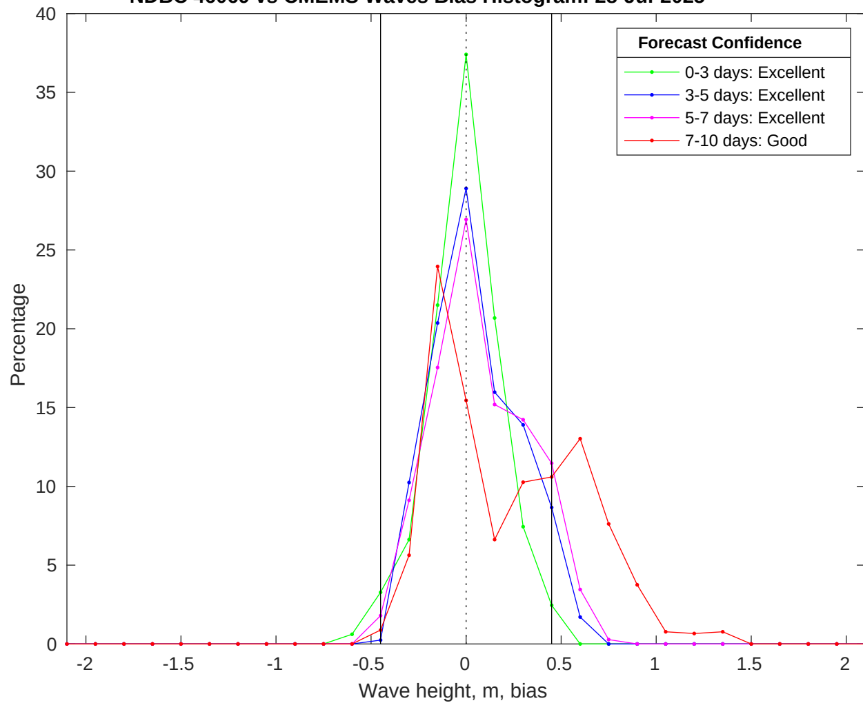
NDBC 46069 vs CMEMS Waves Bias Histogram: 28-Jul-2025
