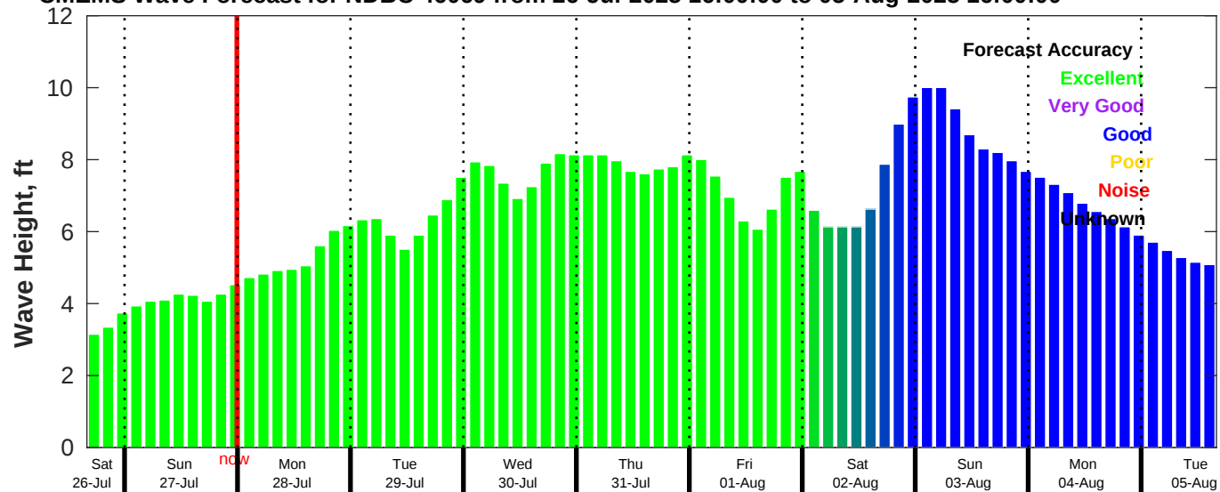
CMEMS Wave Forecast for NDBC 46069 from 26-Jul-2025 16:00:00 to 05-Aug-2025 16:00:00
