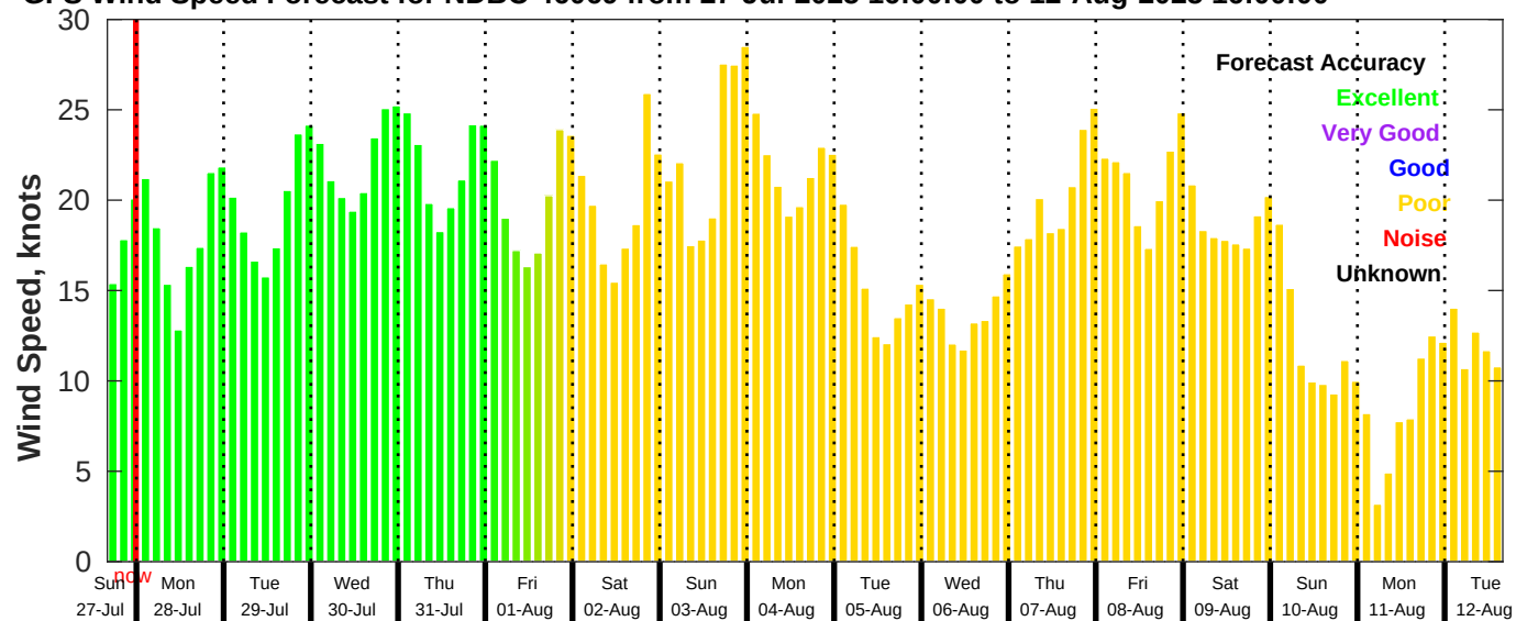
GFS Wind Speed Forecast for NDBC 46069 from 27-Jul-2025 16:00:00 to 12-Aug-2025 16:00:00
