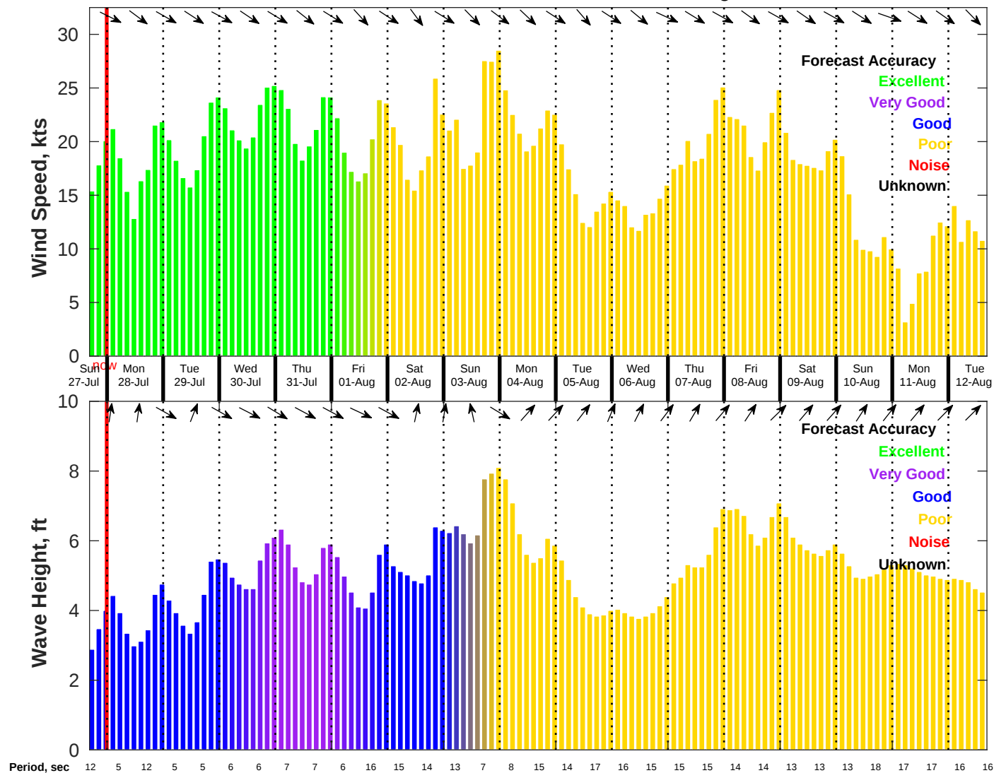
Wind & Wave Forecast for NDBC 46069 from 27-Jul-2025 16:00:00 to 12-Aug-2025 16:00:00
