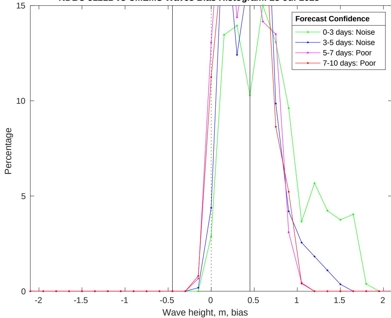
NDBC 51211 vs CMEMS Waves Bias Histogram: 28-Jul-2025
