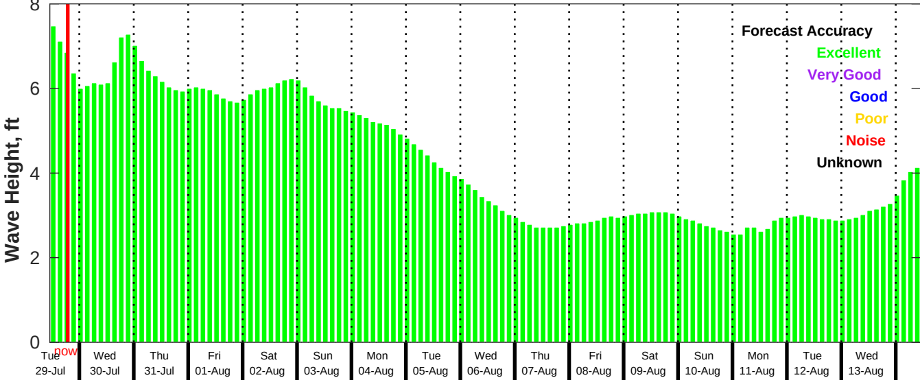
GFS Wave Forecast for NDBC 52211 from 28-Jul-2025 11:00:00 to 13-Aug-2025 11:00:00
